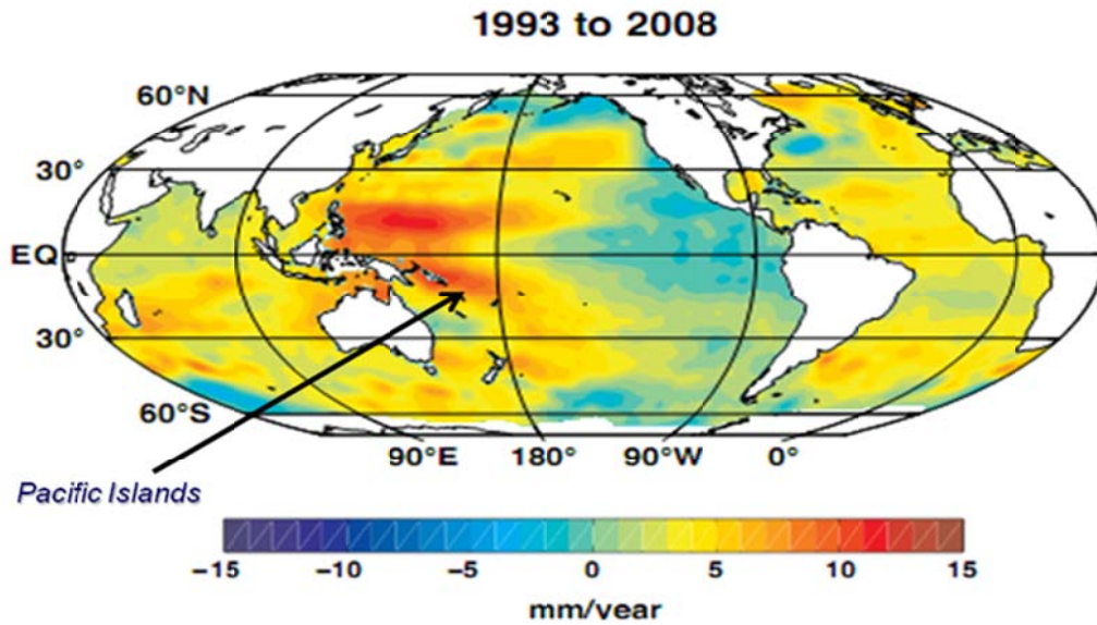
Map 2.1: Geographical pattern of 1993 –2008 sea level trends.
